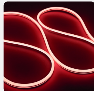
FITA SMD LED NEON 2835 6MM 50M 9,5W/M 120LEDs/M IP65 IRC80 SINGLE SIDE VERMELHO
