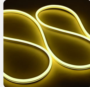
FITA SMD LED NEON 2835 6MM 50M 9,5W/M 120LEDs/M IP65 IRC80 SINGLE SIDE AMARELA
