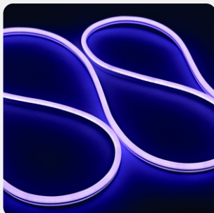
FITA SMD LED NEON 2835 6MM 50M 9,5W/M 120LEDs/M IP65 IRC80 SINGLE SIDE AZUL
