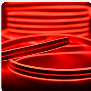
FITA SMD LED NEON 2835 15MM 50M 8W/M 120 LEDS/M IP66 IRC70 DOUBLE SIDE VERMELHA
