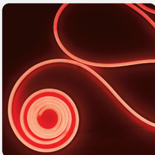
FITA SMD LED NEON 2835 8mm SINGLE SIDE VERMELHA 5M 120LEDs/M IP65 181.12.0147 · 220V · 7W/m FLN2835-8-5-VM-2B
