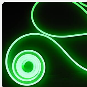
FITA SMD LED NEON 2835 8mm SINGLE SIDE VERDE 5M 120LEDs/M IP65 181.12.0151 · 220V · 7W/m FLN2835-8-5-VD-2B
